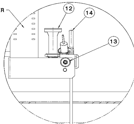
PILOT DETAIL
